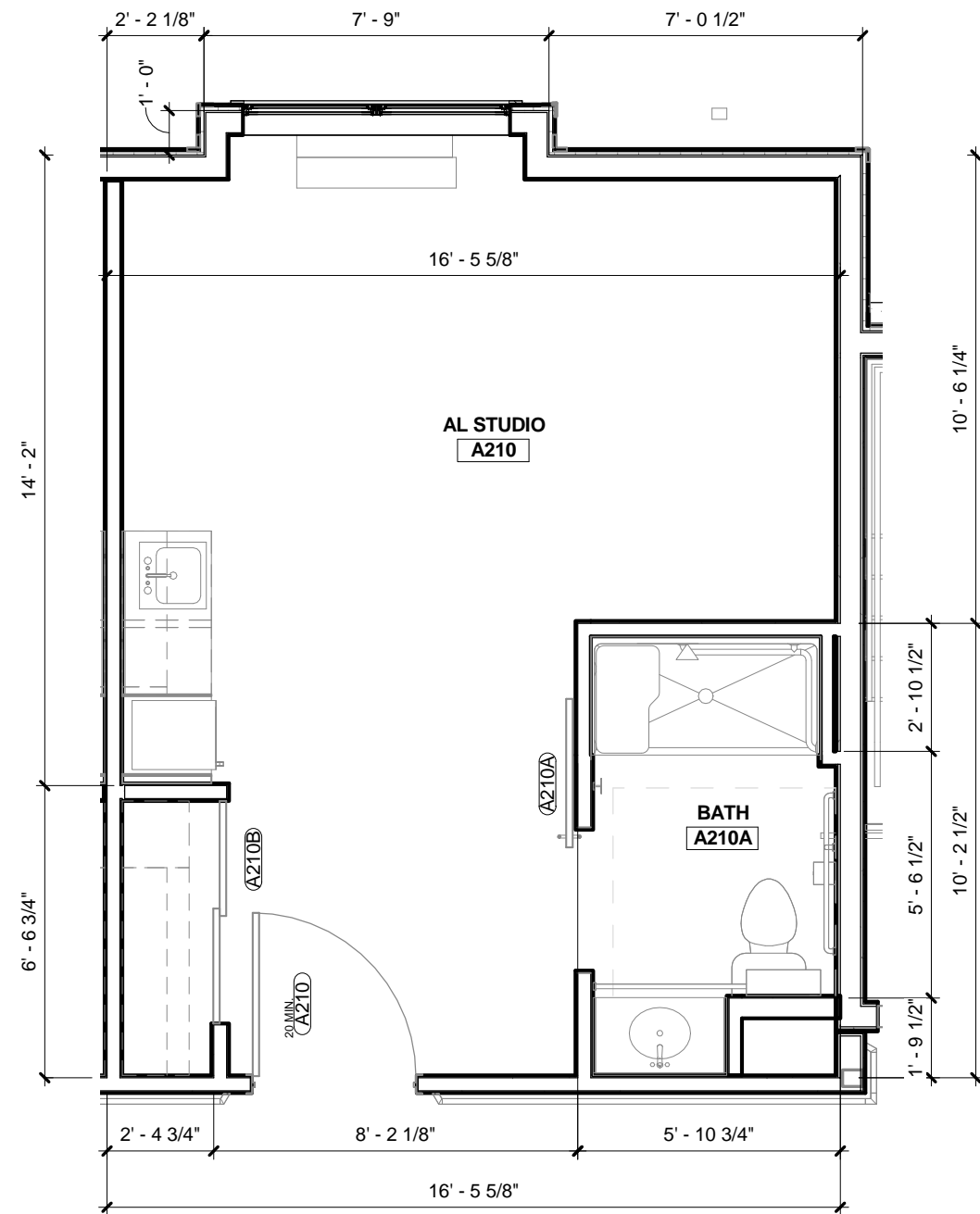
1 AL STUDIO - TYPICAL 1/4" = 1'-0" REFERENCE: 1 / AF2A0
